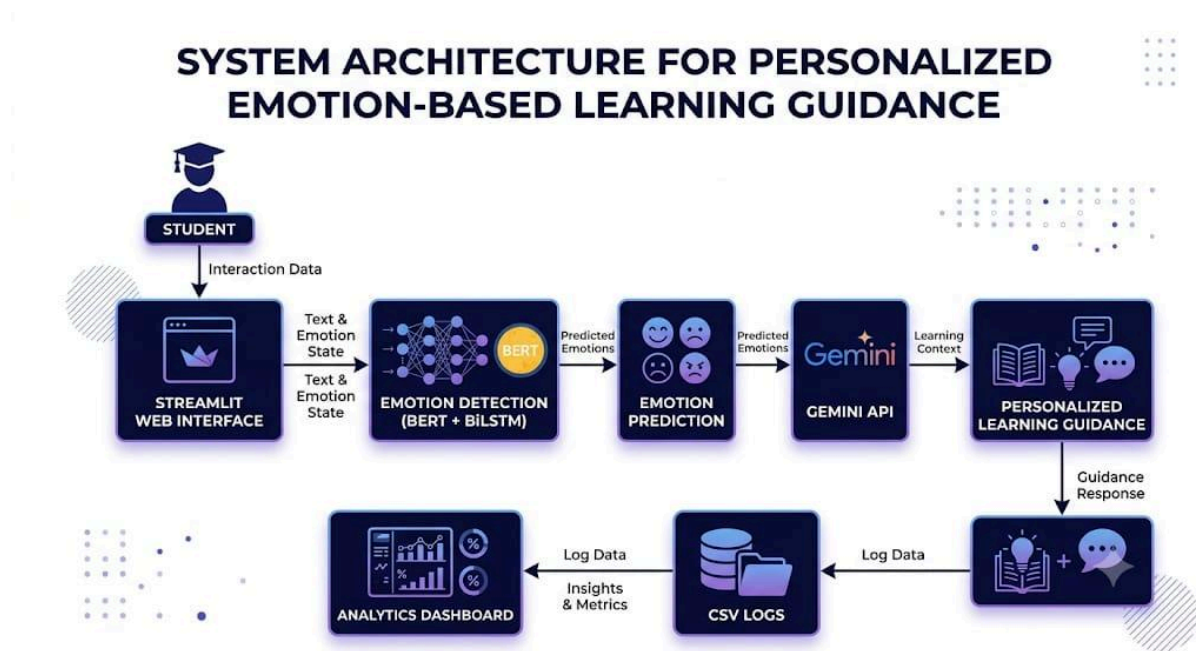
Figure 1: Architecture of the emotion based learning guidance
